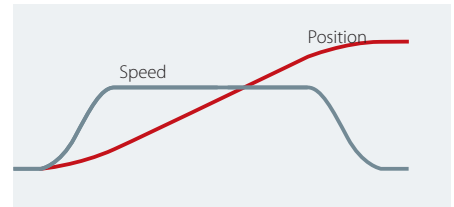
Fig. 2. Motion profile with S-ramps
